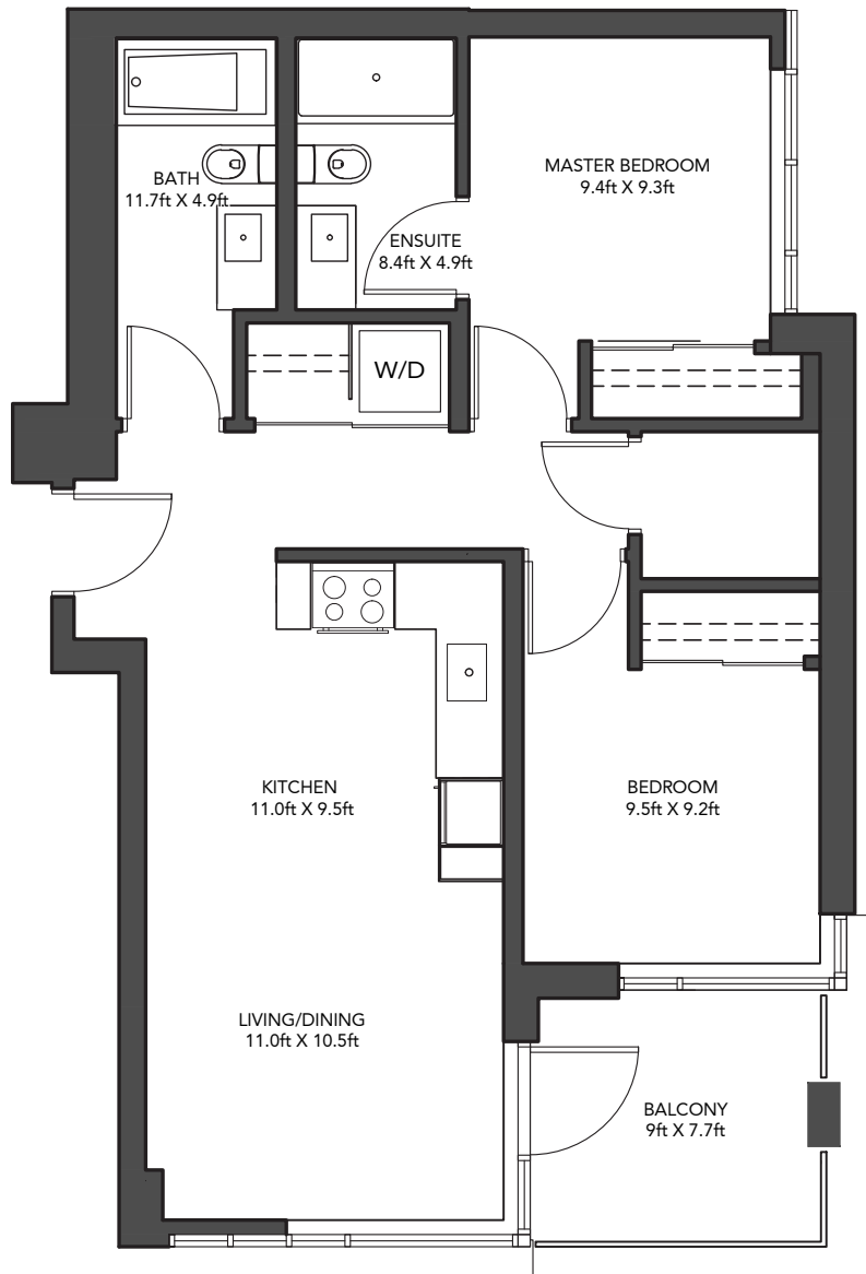
FLOOR PLANS: 1904, 2004, 2104, 2204, 2304
