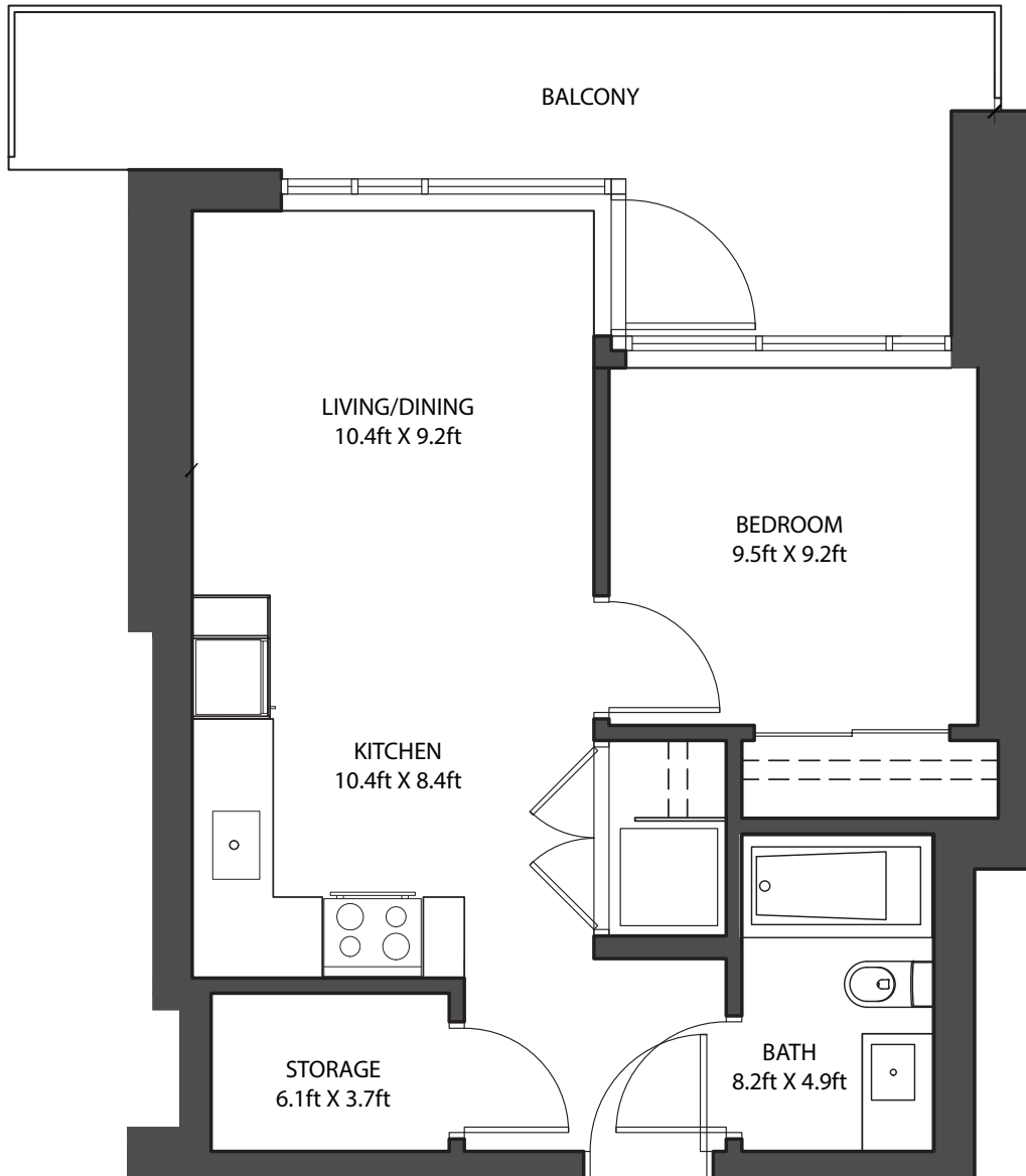
FLOOR PLAN: 302
