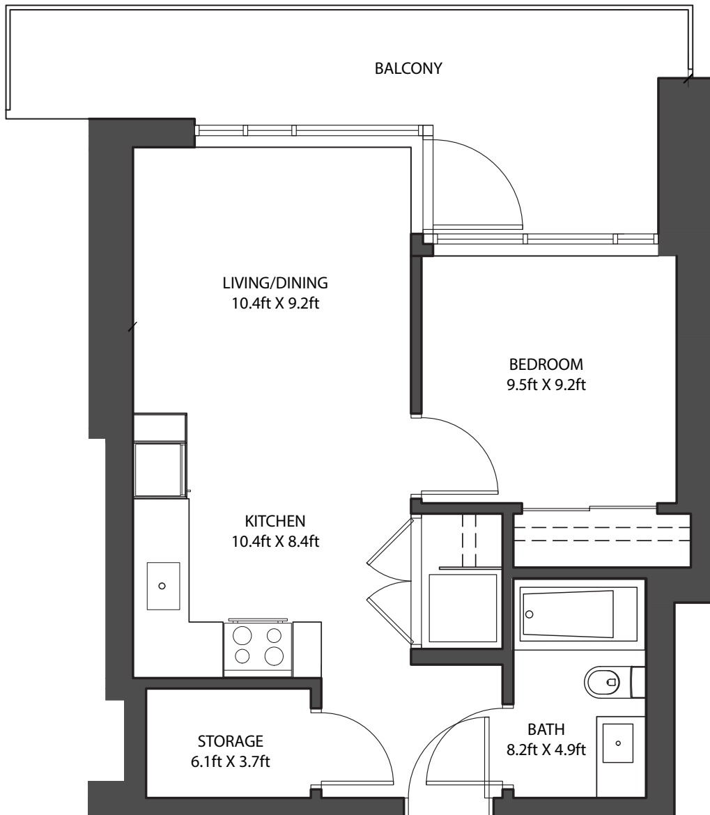
FLOOR PLAN: 302
